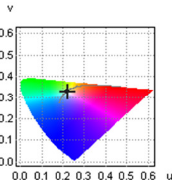
CIE 1960
